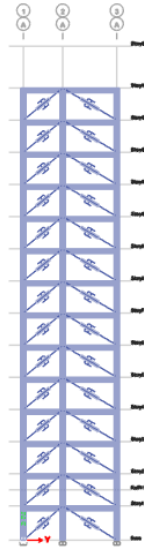
Fig. 8: With Dampers Side View
