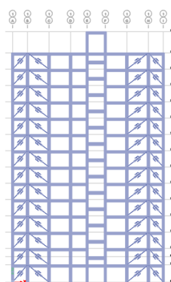
Fig. 4: Front Elevation View
