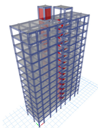
Fig. 1: Without Dampers 3D View
