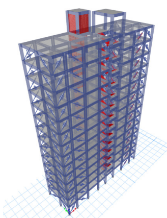
Fig. 3: With Dampers 3D View
