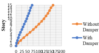
Fig. 9: Storey Displacements of Original and Retrofitted Building
