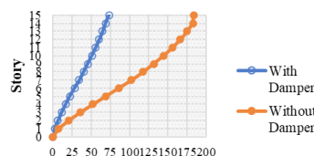
Fig. 10: Storey Displacements of Original and Retrofitted Building
